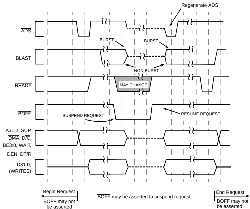
Figure 42. \overline{\text{BOFF}} Functional Timing
