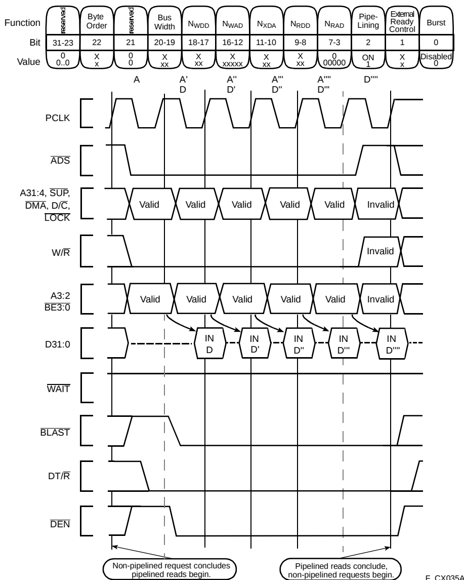
Figure 34. Non-Burst, Pipelined Read Request Without Wait States, 32-Bit Bus
