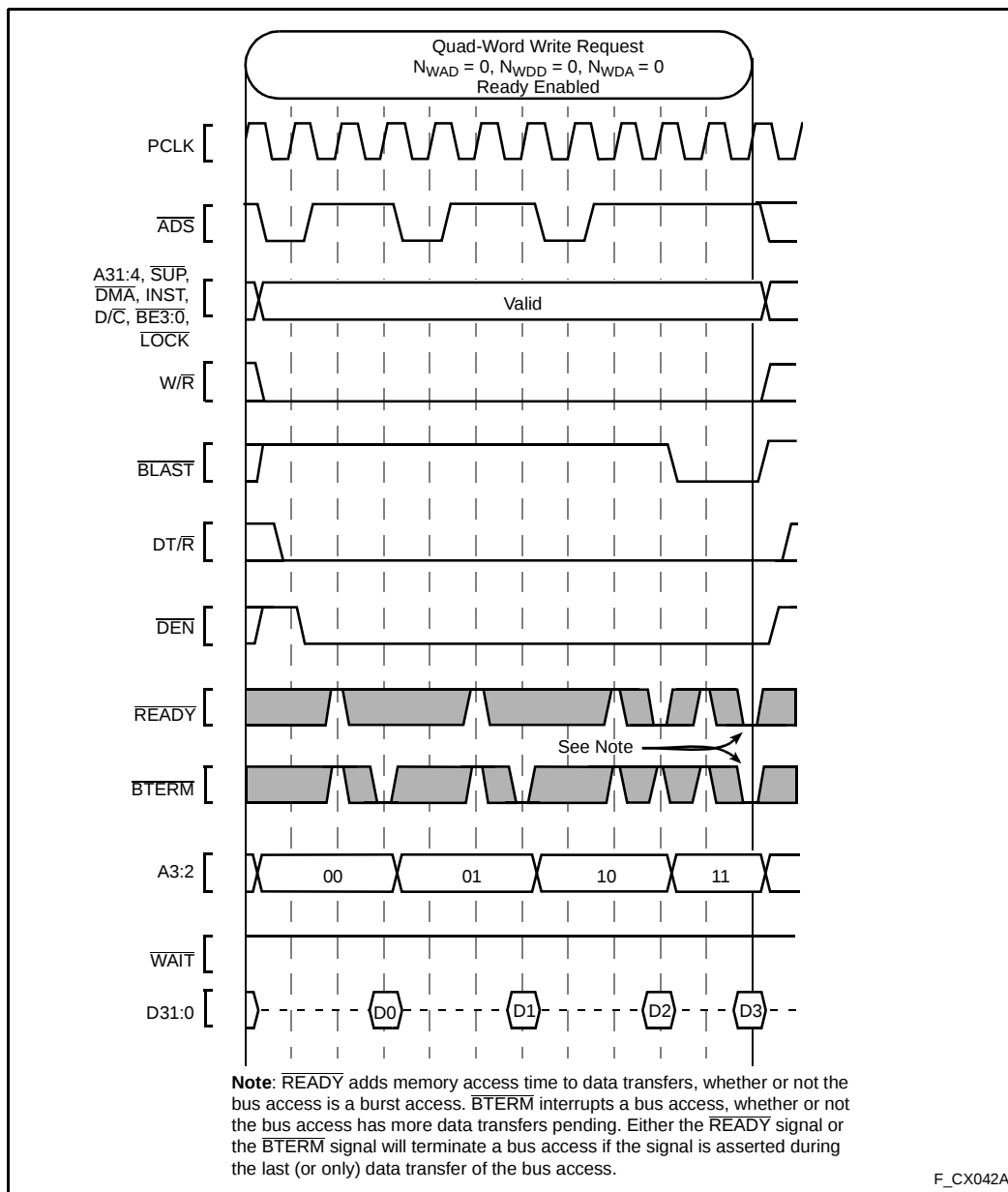
Figure 41. Terminating a Burst with \overline{\text{BTERM}}
