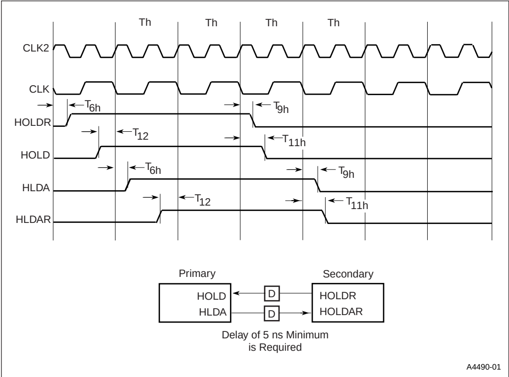
Figure 18. HOLD Timing
