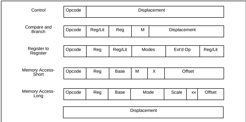
Figure 2. Instruction Formats
