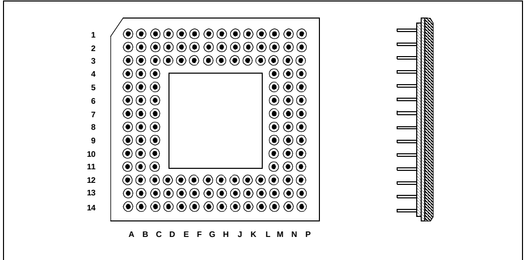
Figure 19. 132-Lead Pin-Grid Array (PGA) Package
