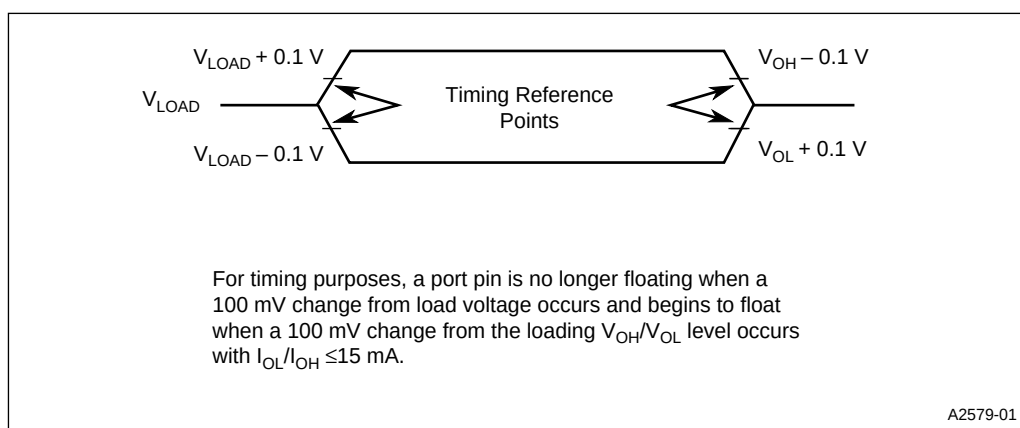
Figure 14. Float Waveforms
