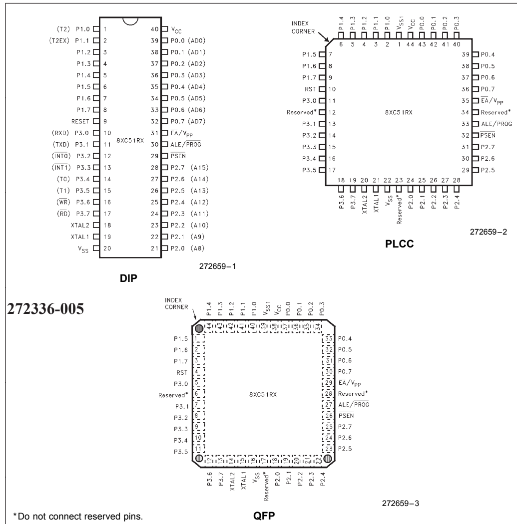
Figure 2. Pin Connections
