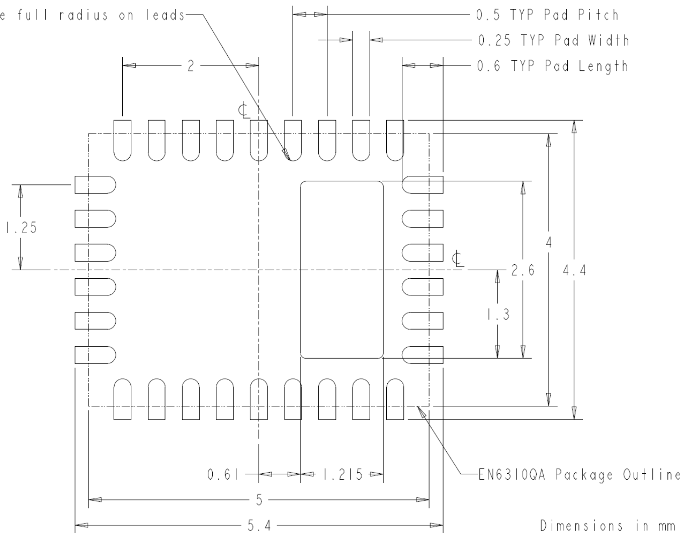
Figure 10: EN6310QA PCB Footprint (Top View)
