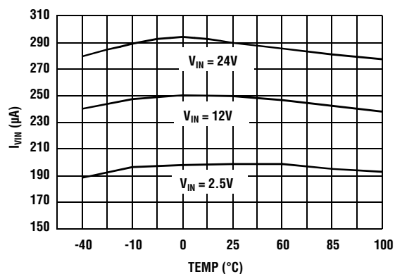
FIGURE 5. V_{IN} CURRENT
