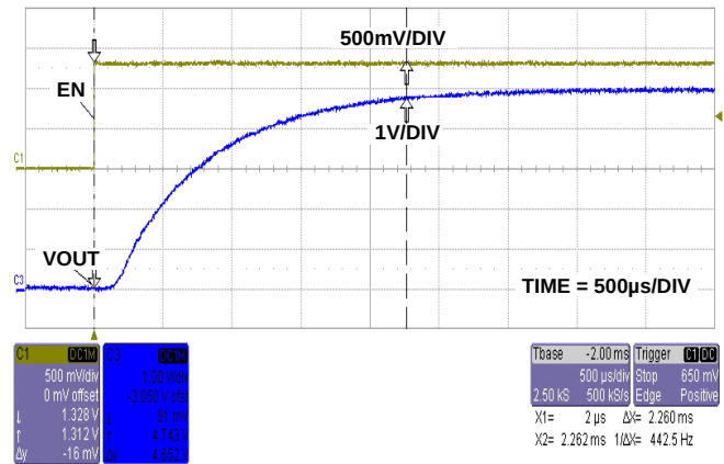
FIGURE 8. START-UP WAVEFORM
