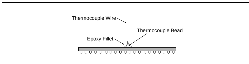
Figure 5. Thermocouple Attachment
