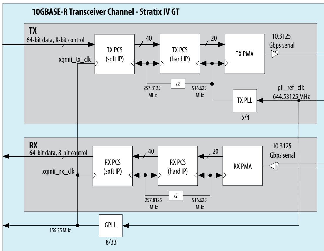
Figure 3-9: Stratix IV Clock Generation and Distribution
