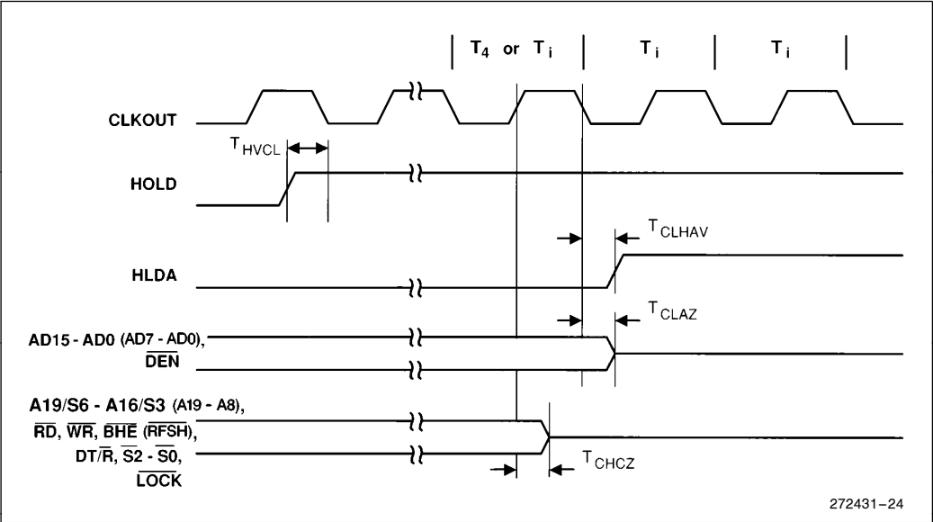
Figure 15. HOLD/HLDA Waveforms (Entering Hold)
