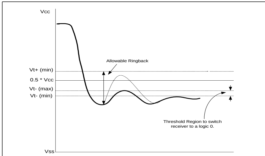
Figure 29. High-to-Low System Bus Receiver Ringback Tolerance for PWRGOOD and TAP Buffers
