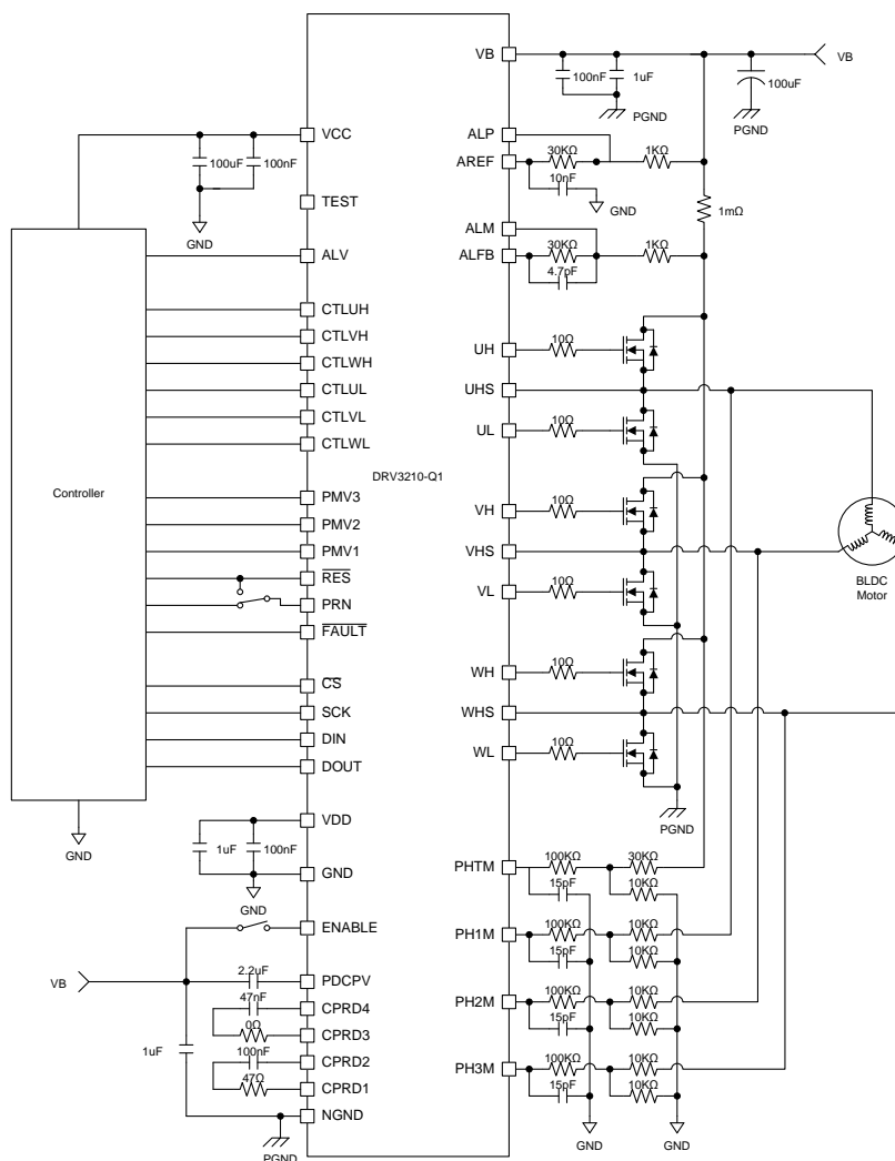
Figure 27. Typical Application Schematic
