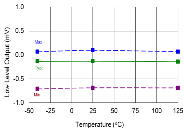
Figure 15. Low Level Output Voltage vs. Temperature
