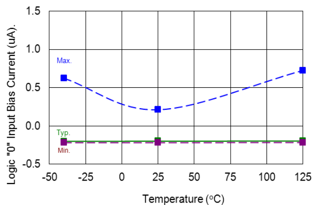
Figure 19. Logic "0" Input Bias Current vs. Temperature
