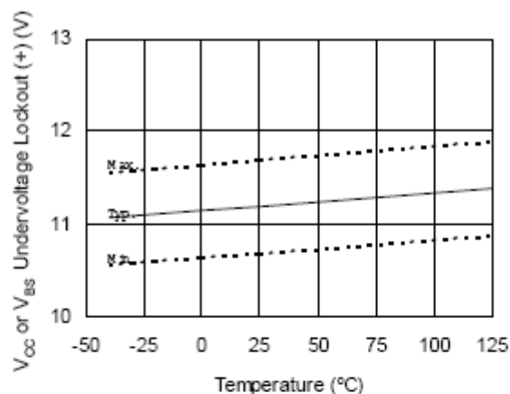
Figure 24. V_{CC} or V_{SS} Undervoltage (+) vs. Temperature (IR21363/21365/IR21366/IR21367 Only)
