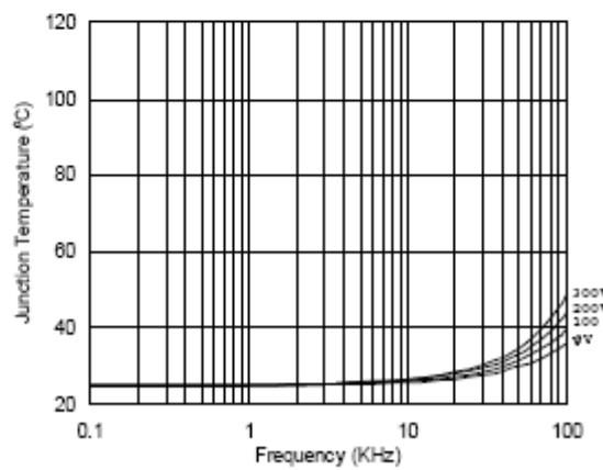
Figure 43. IR2136/IR21362(3)(5)(6)(7)(8) vs. Frequency (IRG4BC40W), R_{gate}=10\Omega , V_{cc}=15V
