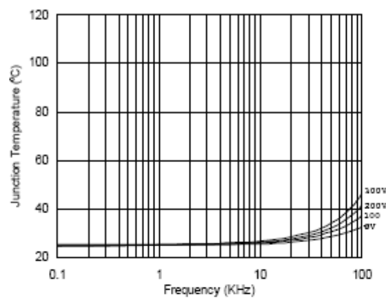
Figure 50. IR2136/IR21362(3)(5)(6)(7)(8) (S) vs. Frequency (IRG4BC30W), R_{gate}=15\Omega , V_{cc}=15V
