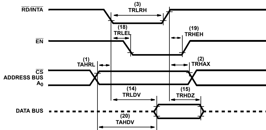
FIGURE 13. READ/INTA
