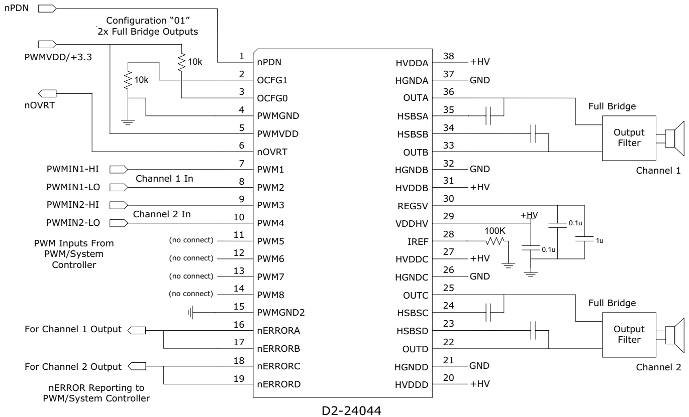
FIGURE 15. 2-CHANNEL FULL BRIDGE EXAMPLE
