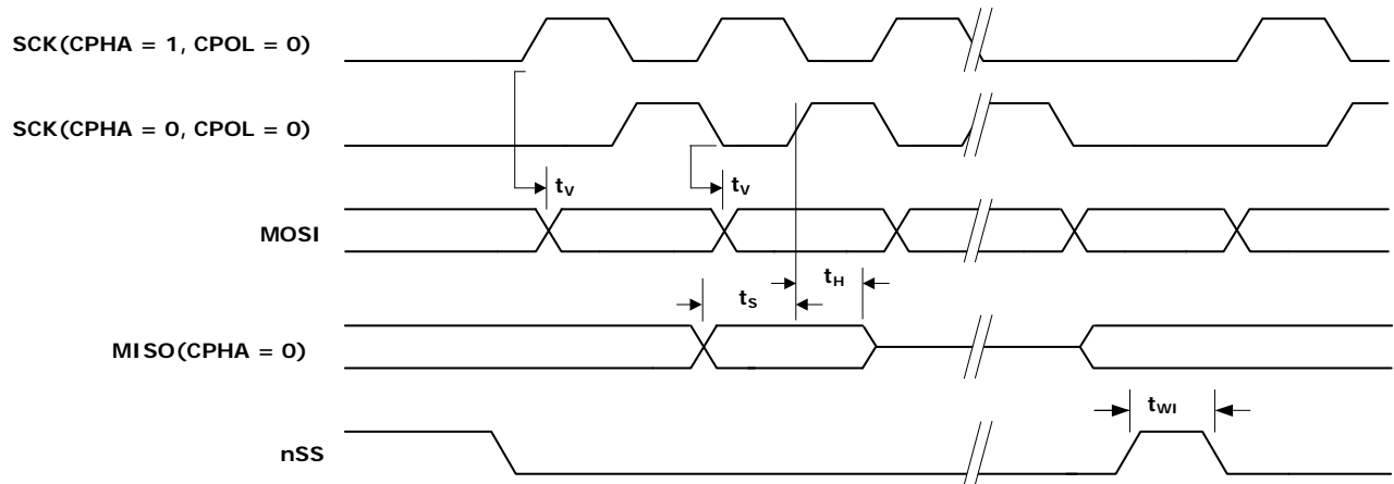
FIGURE 3. SPI TIMING
