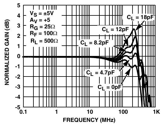
FIGURE 10. GAIN vs FREQUENCY FOR VARIOUS C_{LOAD} ( A_V = +5 )
