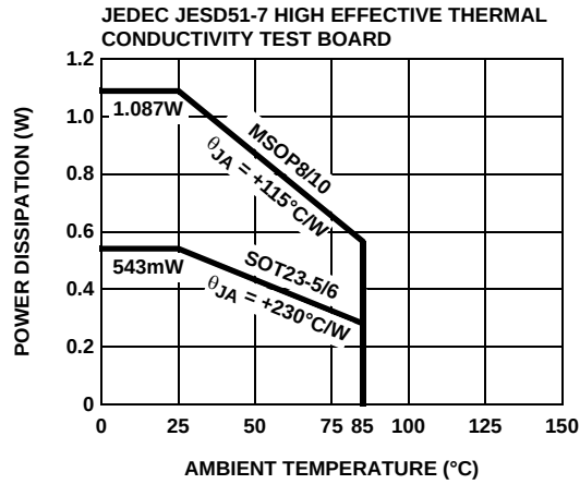
FIGURE 37. PACKAGE POWER DISSIPATION vs AMBIENT TEMPERATURE
