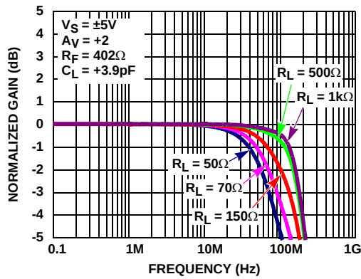
FIGURE 9. GAIN vs FREQUENCY FOR VARIOUS R_{LOAD} ( A_V = +2 )
