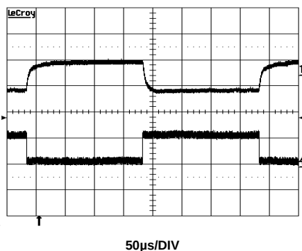
FIGURE 22. V_{ON} TRANSIENT RESPONSE
