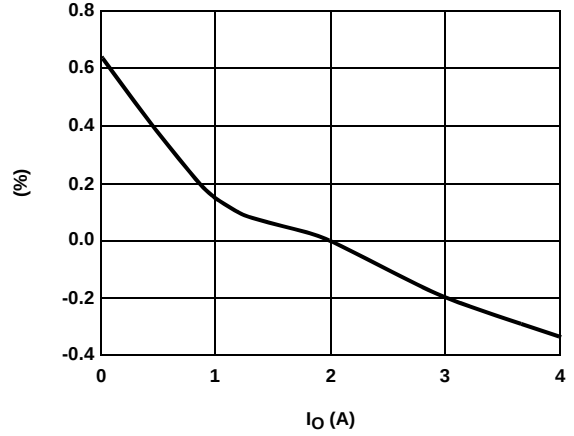
FIGURE 8. LOAD REGULATIONS
