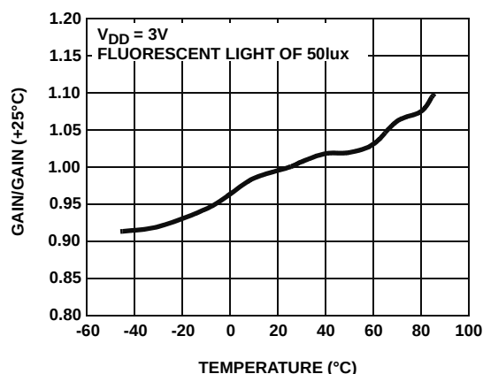
FIGURE 6. GAIN vs TEMPERATURE
