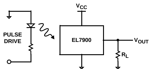
FIGURE 1. RISE/FALL TIME MEASUREMENT Typical Performance Curves
