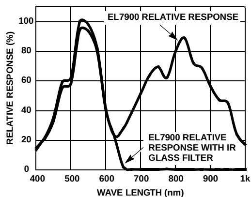
FIGURE 3. SPECTRAL RESPONSE
