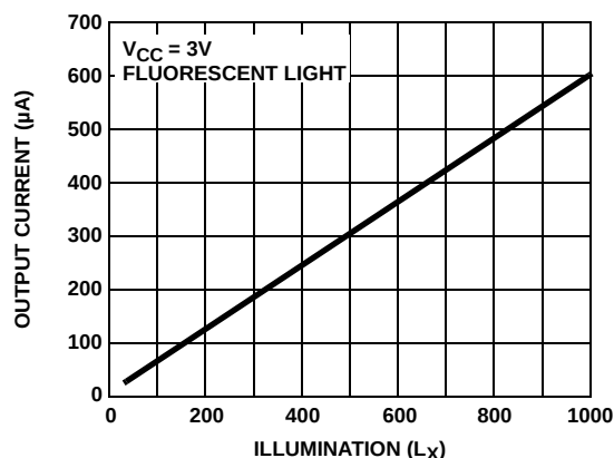
FIGURE 4. SENSITIVITY
