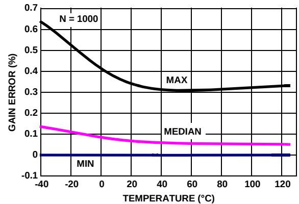
FIGURE 28. EL8173 %GAIN ERROR vs TEMPERATURE, R_L = 100k
