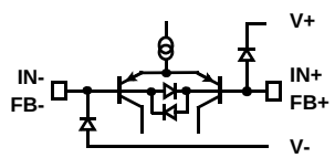
CIRCUIT 1A
