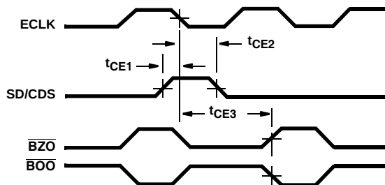
FIGURE 11. ENCODER TIMING
