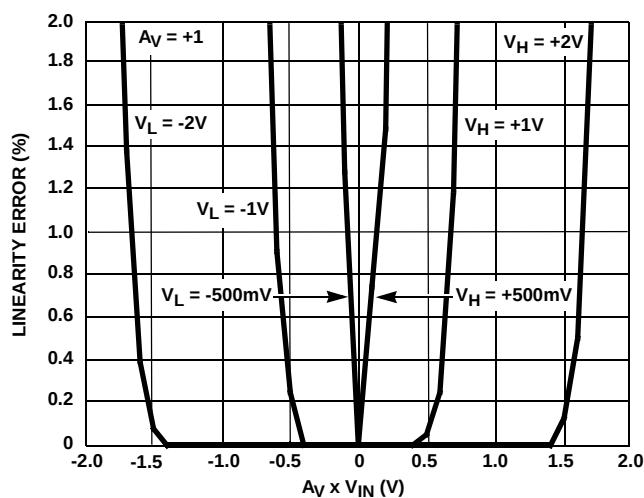
FIGURE 35. LINEARITY NEAR LIMIT VOLTAGE
