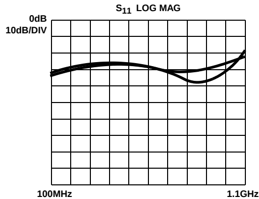
FIGURE 8. RF PORT RETURN LOSS
