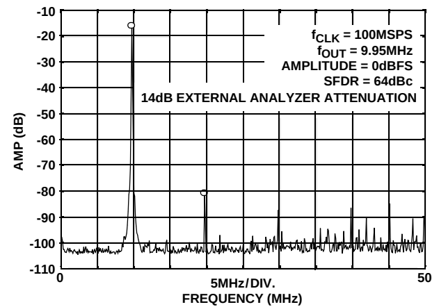
FIGURE 12. SINGLE TONE SFDR
