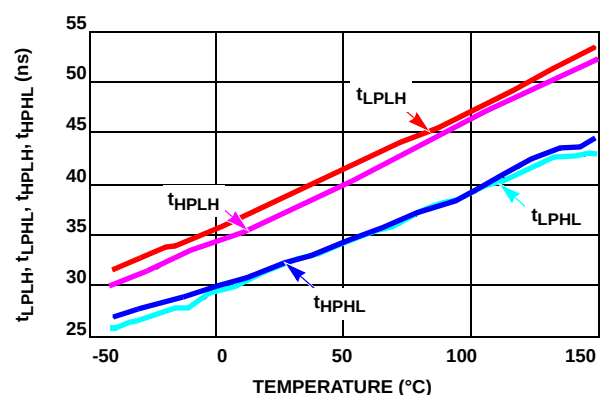
FIGURE 12. HIP2121 PROPAGATION DELAYS vs TEMPERATURE
