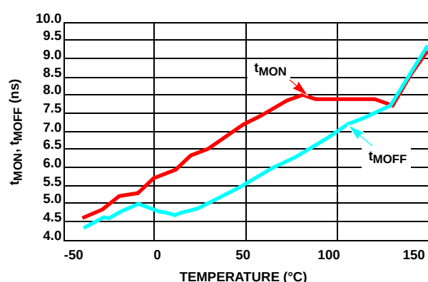
FIGURE 14. HIP2121 DELAY MATCHING vs TEMPERATURE
