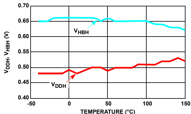
FIGURE 10. UNDERVOLTAGE LOCKOUT HYSTERESIS vs TEMPERATURE
