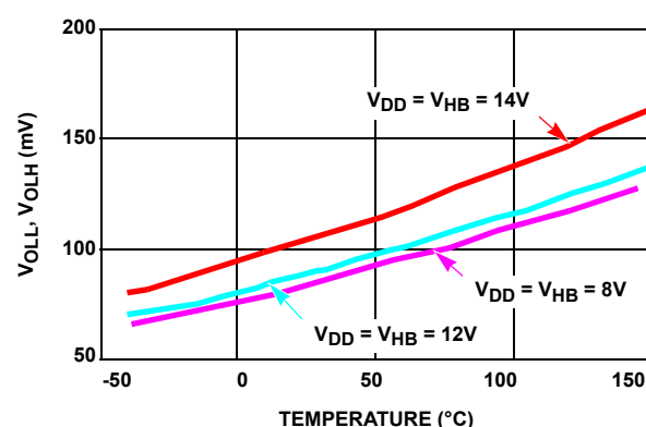
FIGURE 8. LOW LEVEL OUTPUT VOLTAGE vs TEMPERATURE
