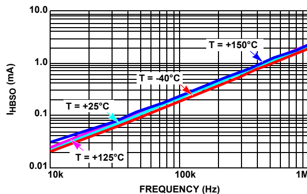
FIGURE 6. I_{HBS} OPERATING CURRENT vs FREQUENCY
