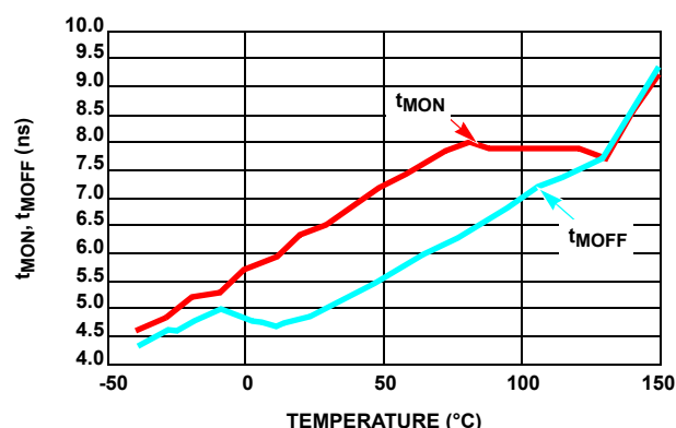
FIGURE 14. HIP2123 DELAY MATCHING vs TEMPERATURE
