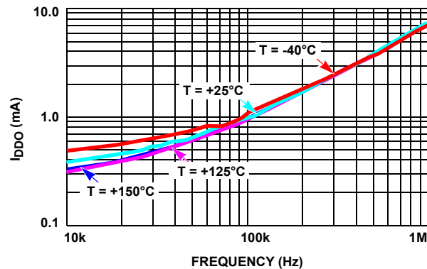
FIGURE 4. HIP2123 I_{DD} OPERATING CURRENT vs FREQUENCY
