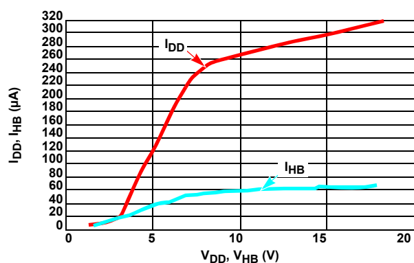
FIGURE 18. HIP2123 QUIESCENT CURRENT vs VOLTAGE
