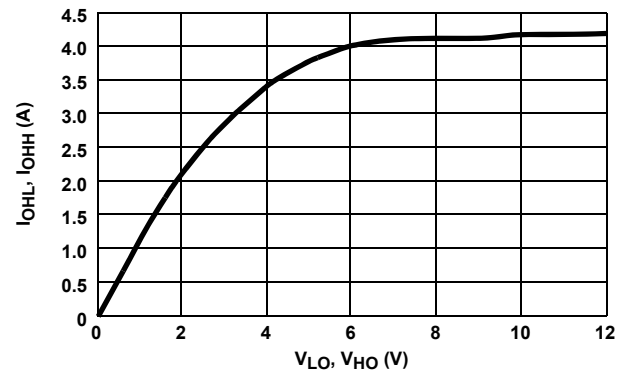
FIGURE 16. PEAK PULL-DOWN CURRENT vs OUTPUT VOLTAGE
