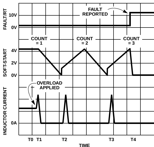
FIGURE 5. OVER-CURRENT OPERATION
