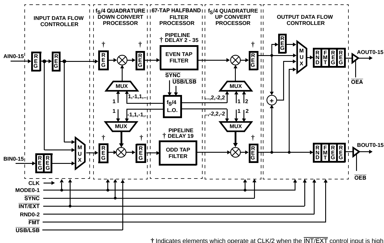
FIGURE 1. HALFBAND BLOCK DIAGRAM
