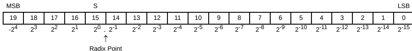
FIGURE 3. BIT WEIGHTING
