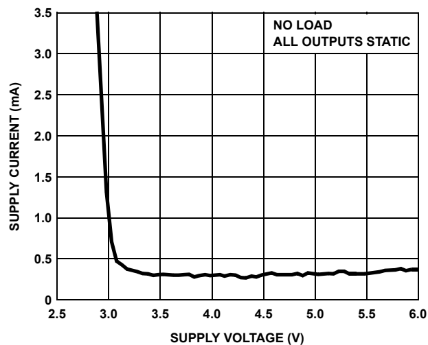
FIGURE 23. SUPPLY CURRENT vs SUPPLY VOLTAGE
