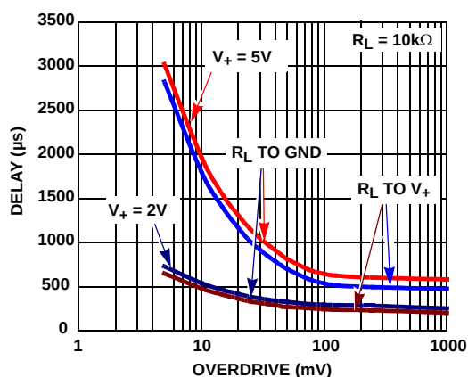
FIGURE 8. ISL28197 PROP DELAY vs OVERDRIVE (RISING EDGE)
