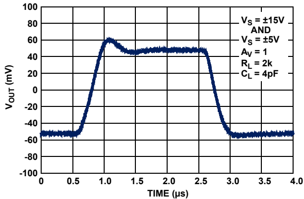
FIGURE 81. CHARACTERIZED SMALL SIGNAL TRANSIENT RESPONSE
