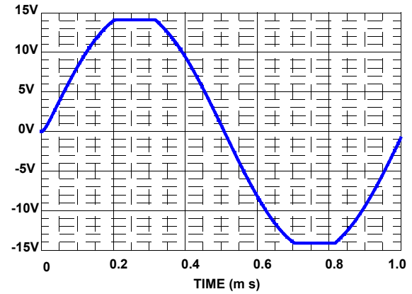
FIGURE 59. SIMULATED OUTPUT VOLTAGE SWING \pm 15V
