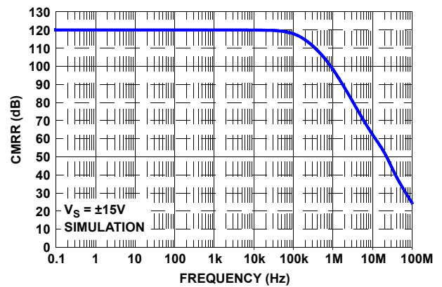
FIGURE 57. SIMULATED (SPICE) CMRR
