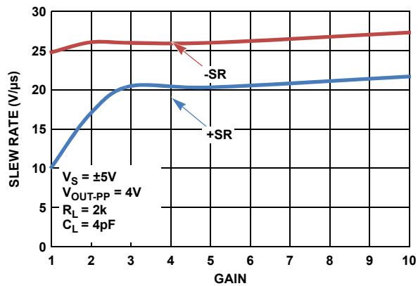
FIGURE 33. SLEW RATE vs NON-INVERTING CLOSED LOOP GAIN, V_S = \pm 5V
