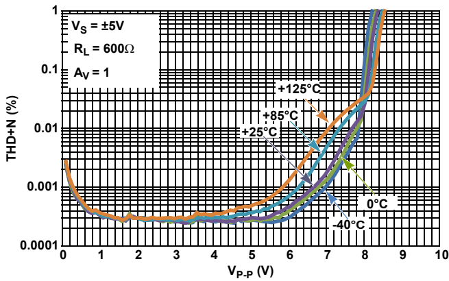
FIGURE 43. UNITY-GAIN THD+N vs OUTPUT VOLTAGE vs TEMPERATURE AT V_S = \pm 5V FOR 600Ω LOAD
