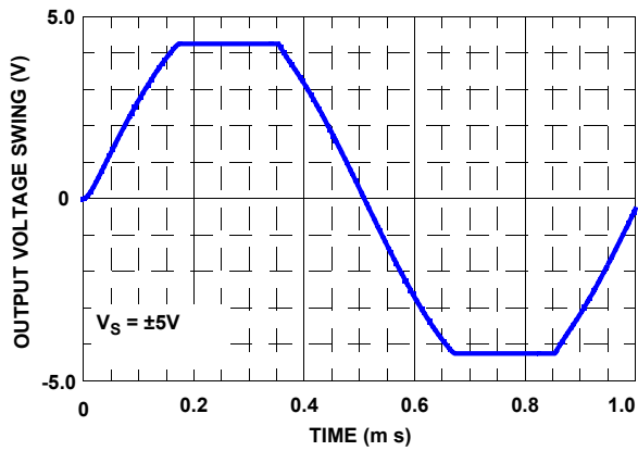
FIGURE 58. SIMULATED OUTPUT VOLTAGE SWING \pm 5V
