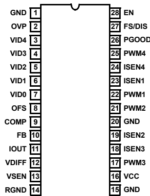
ISL6559CB (28 LEAD SOIC)
