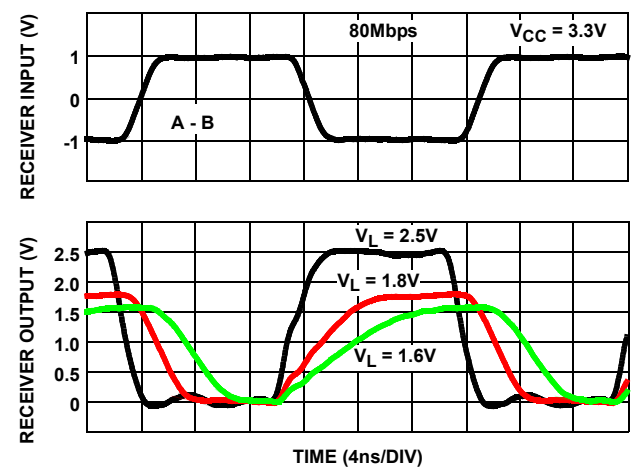
FIGURE 33. ISL32177E RECEIVER WAVEFORMS
