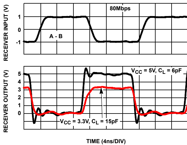
FIGURE 30. ISL3217XE RECEIVER WAVEFORMS
