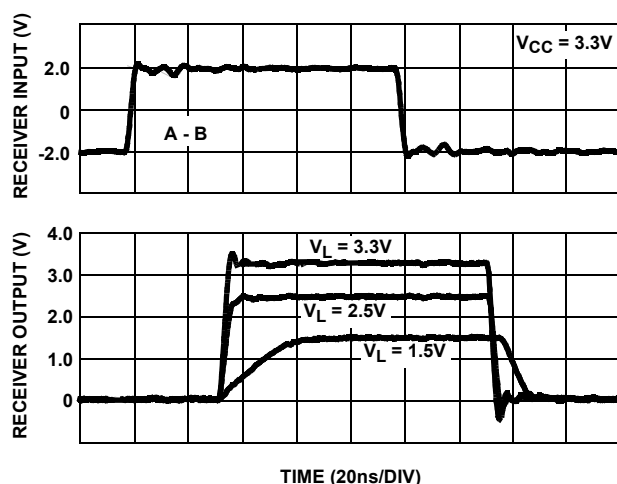
FIGURE 16. RECEIVER WAVEFORMS
