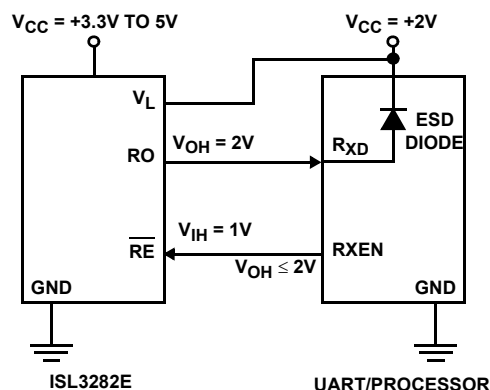
FIGURE 3. USING V_L PIN TO ADJUST LOGIC LEVELS
