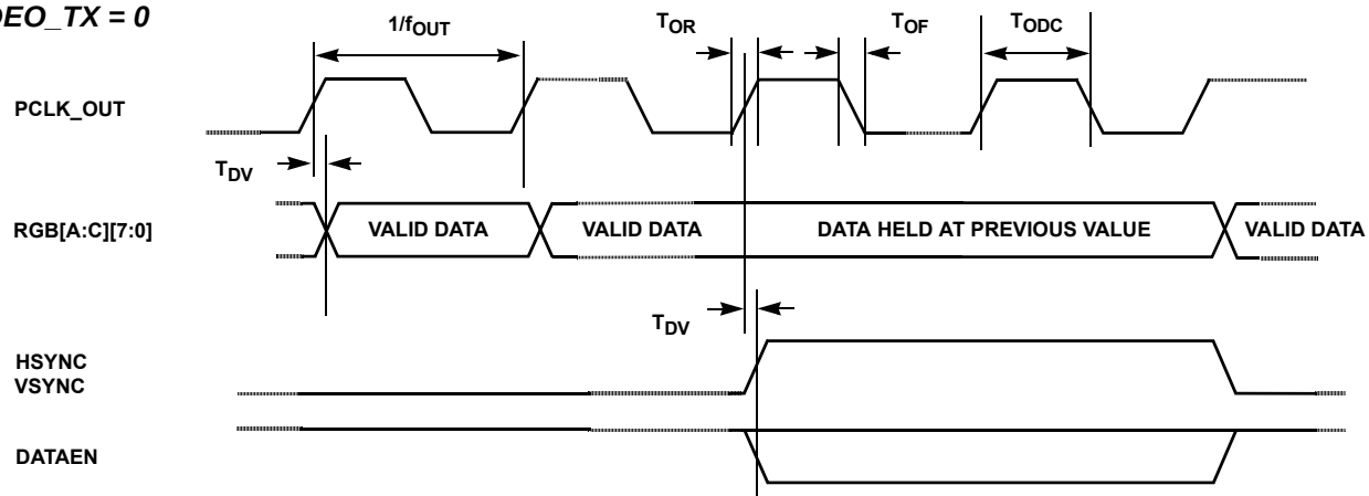
FIGURE 3. PARALLEL VIDEO OUTPUT TIMING [PCLK_OUT ACTIVE LOW, HSYNC/VSNC ACTIVE HIGH]
