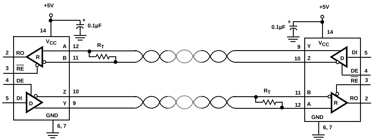
ISL4489E, ISL4491E
