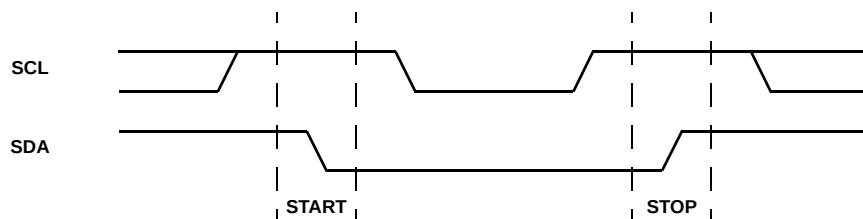
FIGURE 14. VALID START AND STOP CONDITIONS
