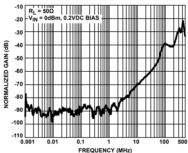
FIGURE 26. CROSSTALK
