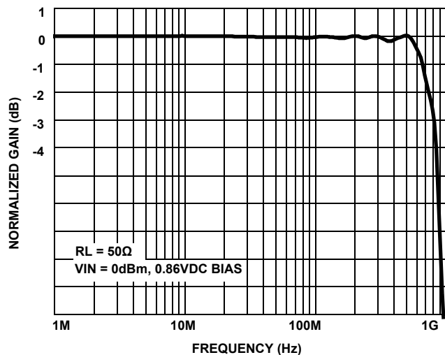
FIGURE 21. FREQUENCY RESPONSE
