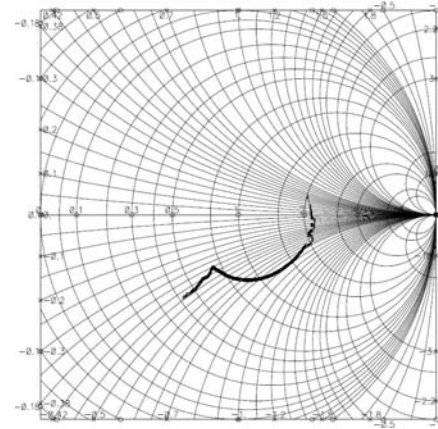
FIGURE 14. SMITH CHART OF S33
