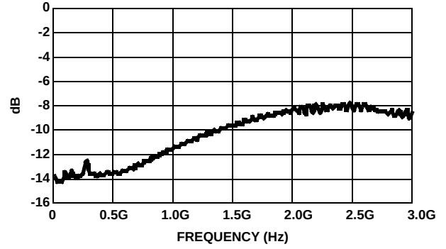
FIGURE 2. |Scs21| vs FREQUENCY
