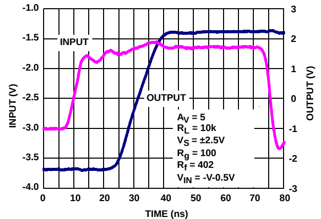
FIGURE 24. NEGATIVE INPUT OVERLOAD RECOVERY TIME
