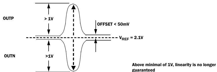
FIGURE 2. OUTP/OUTN
