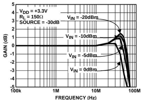
FIGURE 4. FREQUENCY RESPONSE FOR VARIOUS V_{IN}
