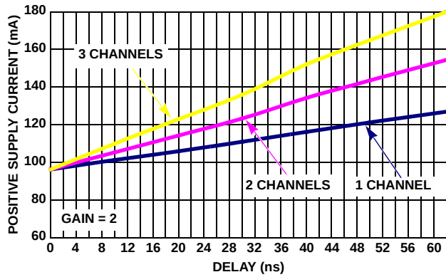
FIGURE 20. ISL59920 POSITIVE SUPPLY CURRENT ( V_{SP} ) vs DELAY TIME
